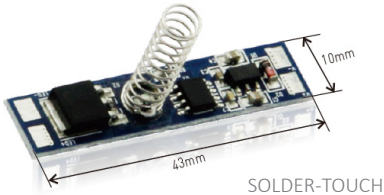
SOLDER-TOUCH
