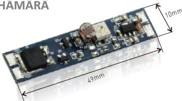
SOLDER-LIGHT-SENSOR
